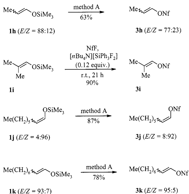
Scheme 4. Method A: [\text{nBu}_4\text{N}]\text{F} (0.15–0.29 equiv.), THF, NfF (1.1–2.0 equiv.), 0 °C \rightarrow room temp., 16–18 h unless otherwise noted
