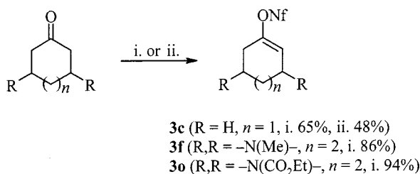
Scheme 6. i. 1) i Pr 2 NLi in THF, -78 °C; 2) NfF, -78 °C → room temp., overnight; ii. DBU in toluene at 85 °C, NfF, 85 °C overnight
