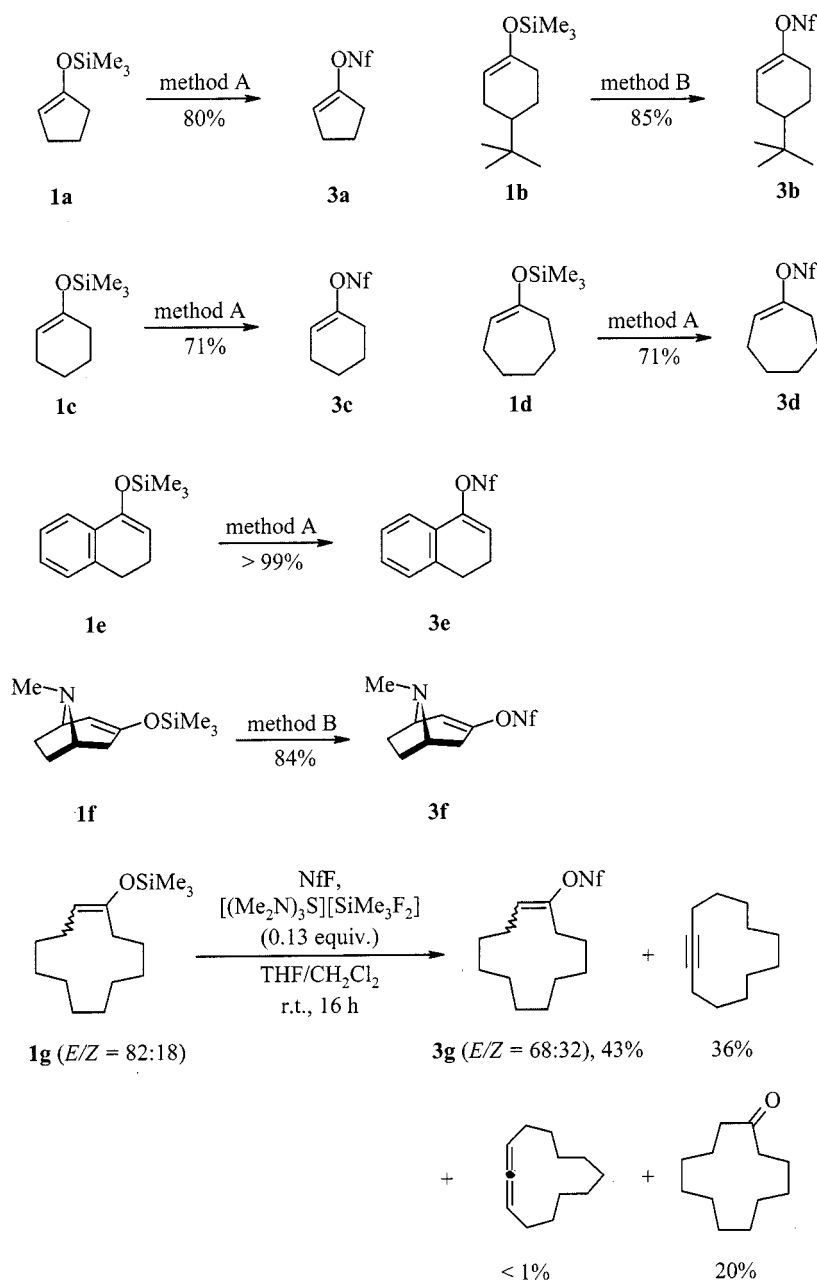
Scheme 3. Method A: [ n Bu 4 N]F (0.15–0.29 equiv.), THF, NfF (1.1–2.0 equiv.), 0 °C → room temp., 16–18 h; Method B: [ n -Bu 4 N]F (0.04–0.05 equiv.), KF, THF, NfF (1.2–1.3 equiv.), –78 °C → room temp., 16–18 h
